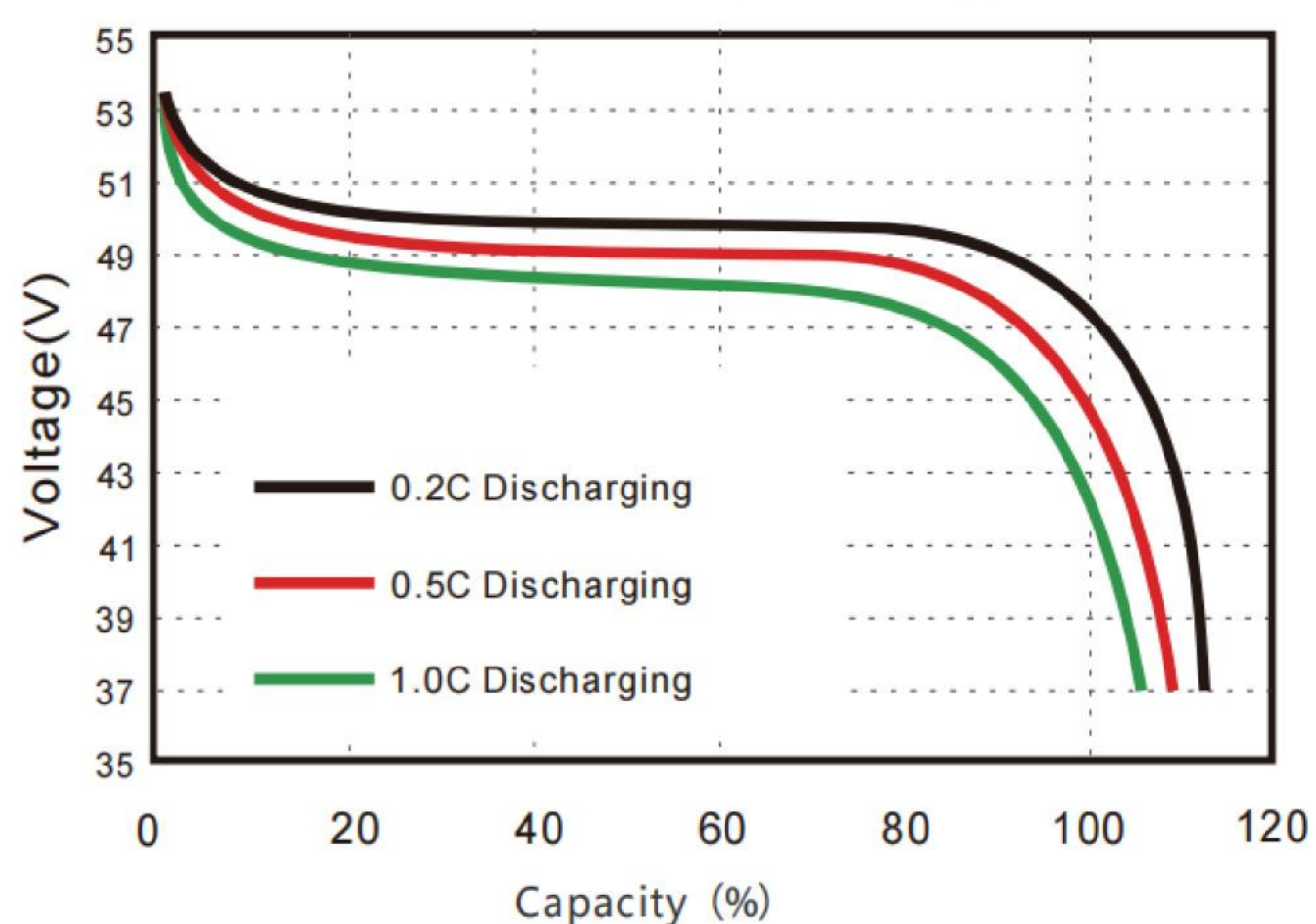
● Different Rate Discharge Curve @25°C
