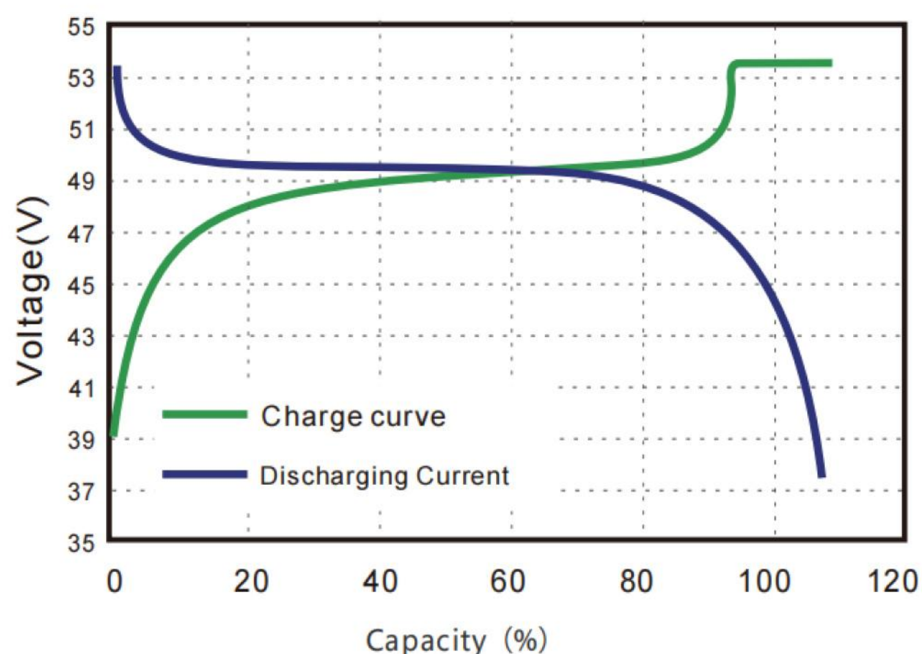
● Charge and discharge curve@0.5C 25°C
