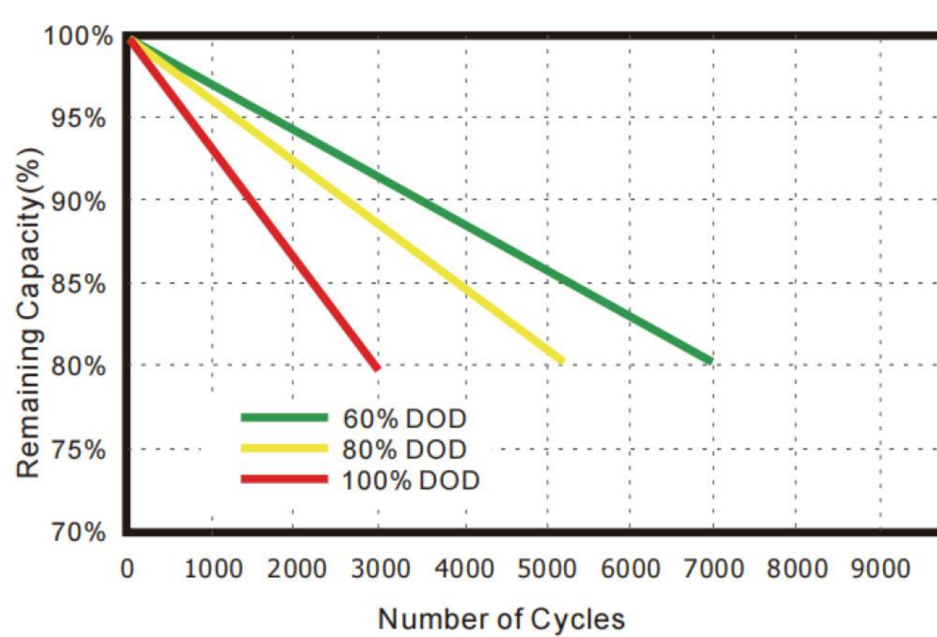
● Different discharge depth life curves & 40°C 0.5C
