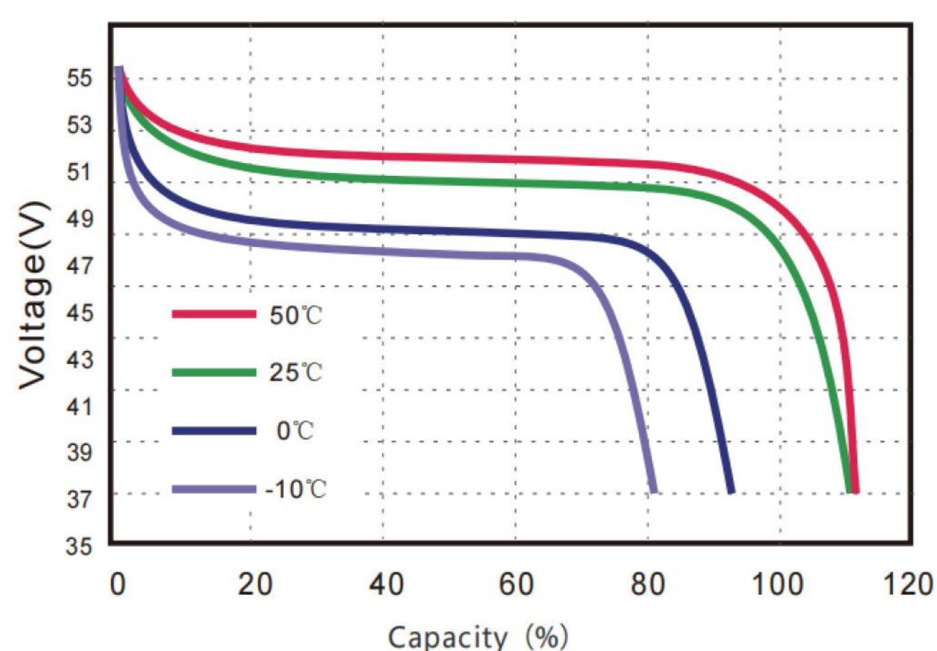
● Different Temperature Discharge Curve @0.5C
