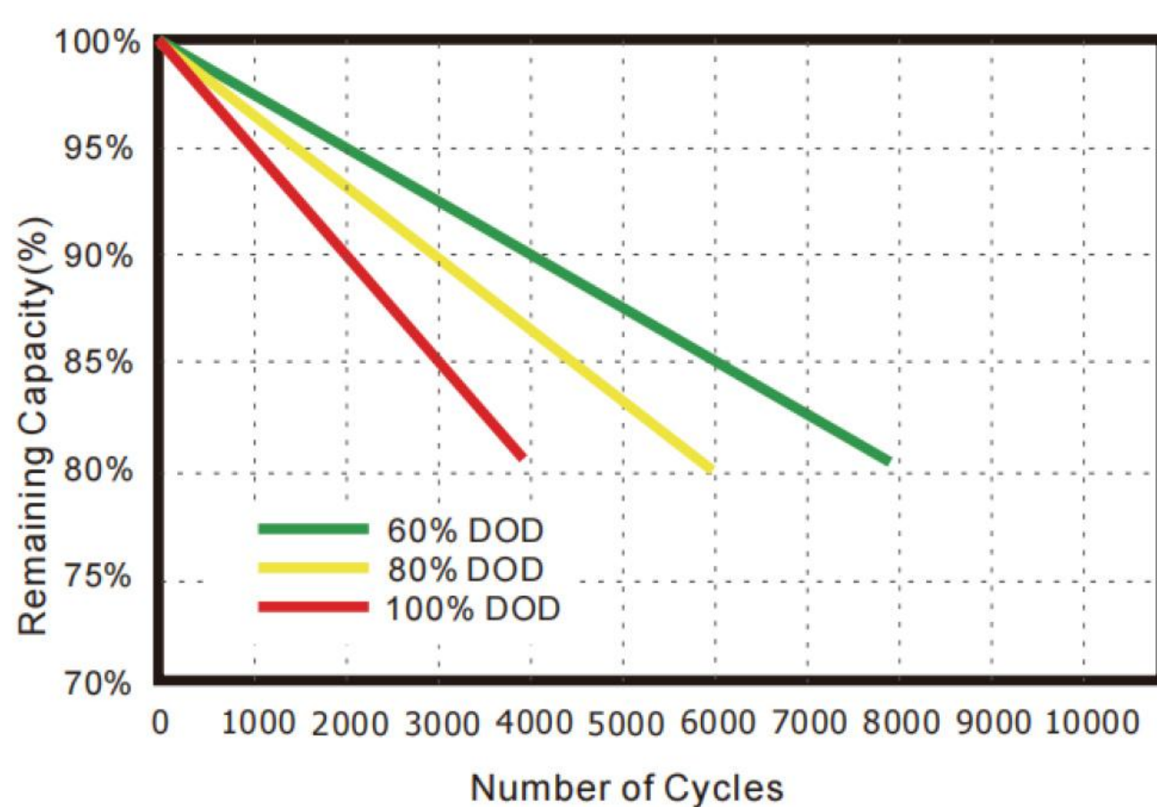
● Different discharge depth life curves & 25°C 0.5C
