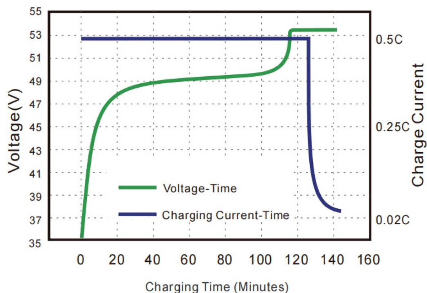
● Charging Characteristics @0.5C 25°C
